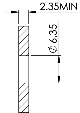
PANEL DETAIL
